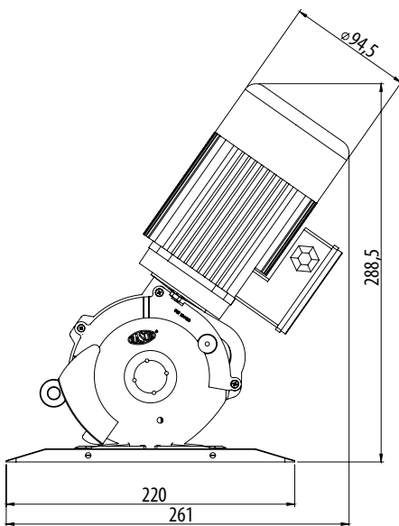
Dimension layout
